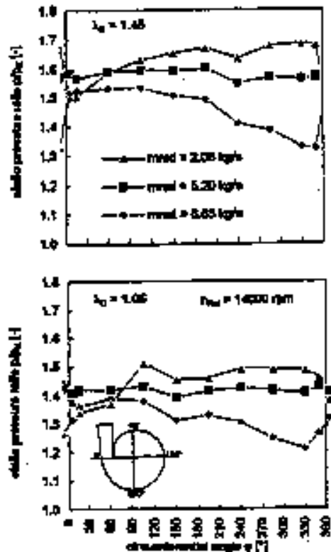
Figure 2. Circumferential static pressure distribution in vaneless diffuser (Hagelstein et al 1997, Fig. 13)
