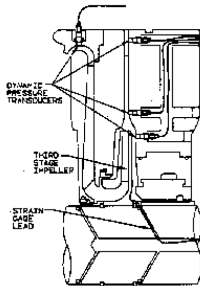
Figure 8. Detail view of dynamic instrumentation for stage 3 of 6 in test rig.
