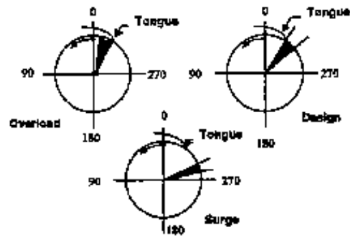
Figure 19. Circumferential location of peak dynamic strain.
