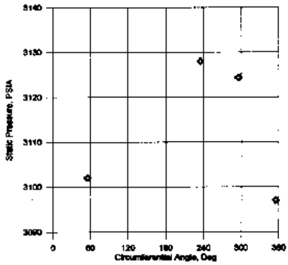
Figure 15. Impeller inlet circumferential static pressure distribution for stage 3 of 6 in test rig, data point 15.
