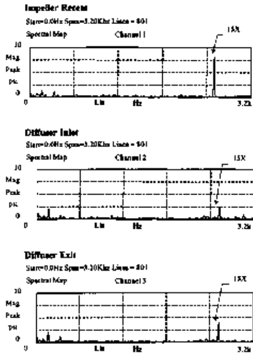
Figure 16. Dynamic pressure response for stage 3 of 6 in test rig, data point 18.
